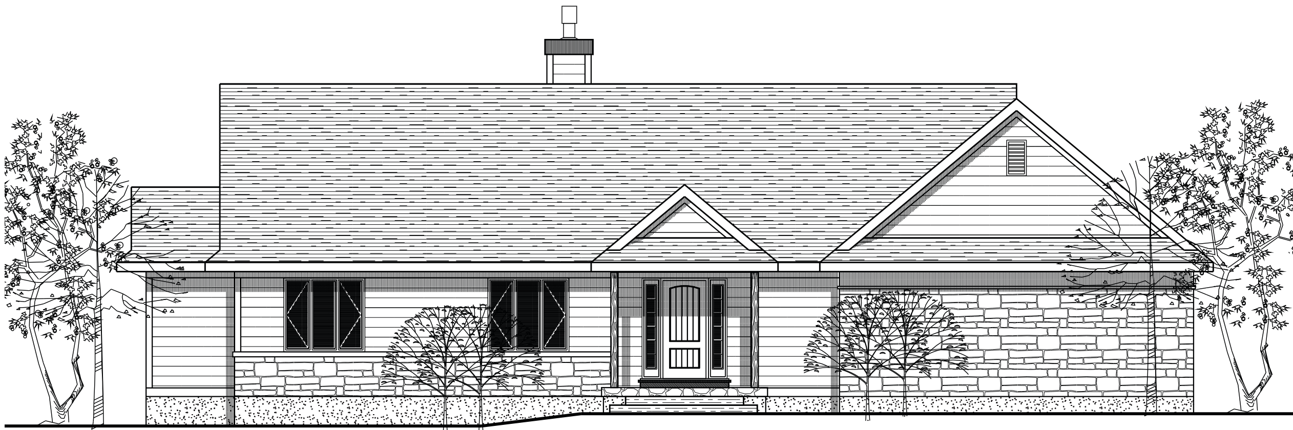
FRONT ELEVATION
