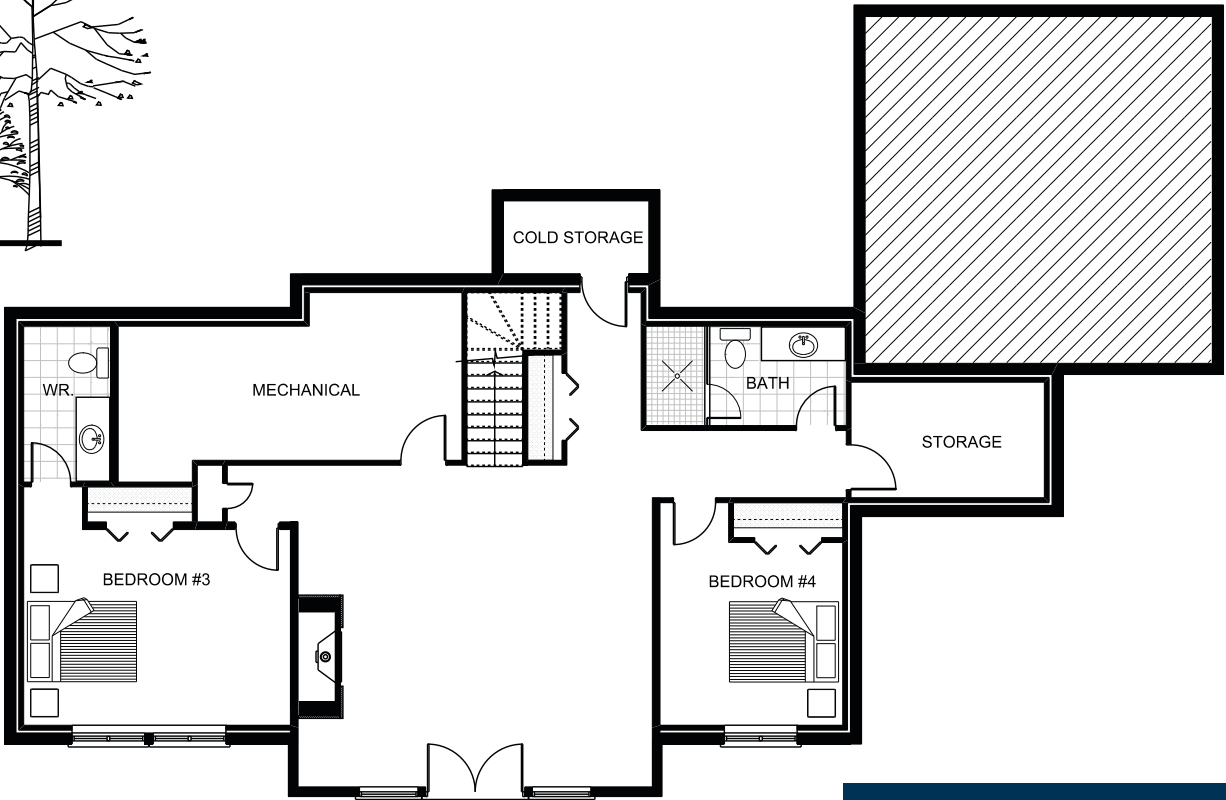
SUGGESTED LOWER FLOOR PLAN
