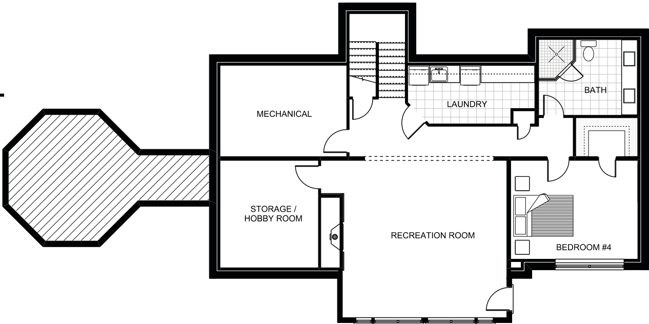
SUGGESTED LOWER FLOOR PLAN
