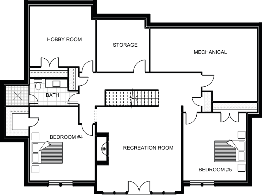
SUGGESTED LOWER FLOOR PLAN
