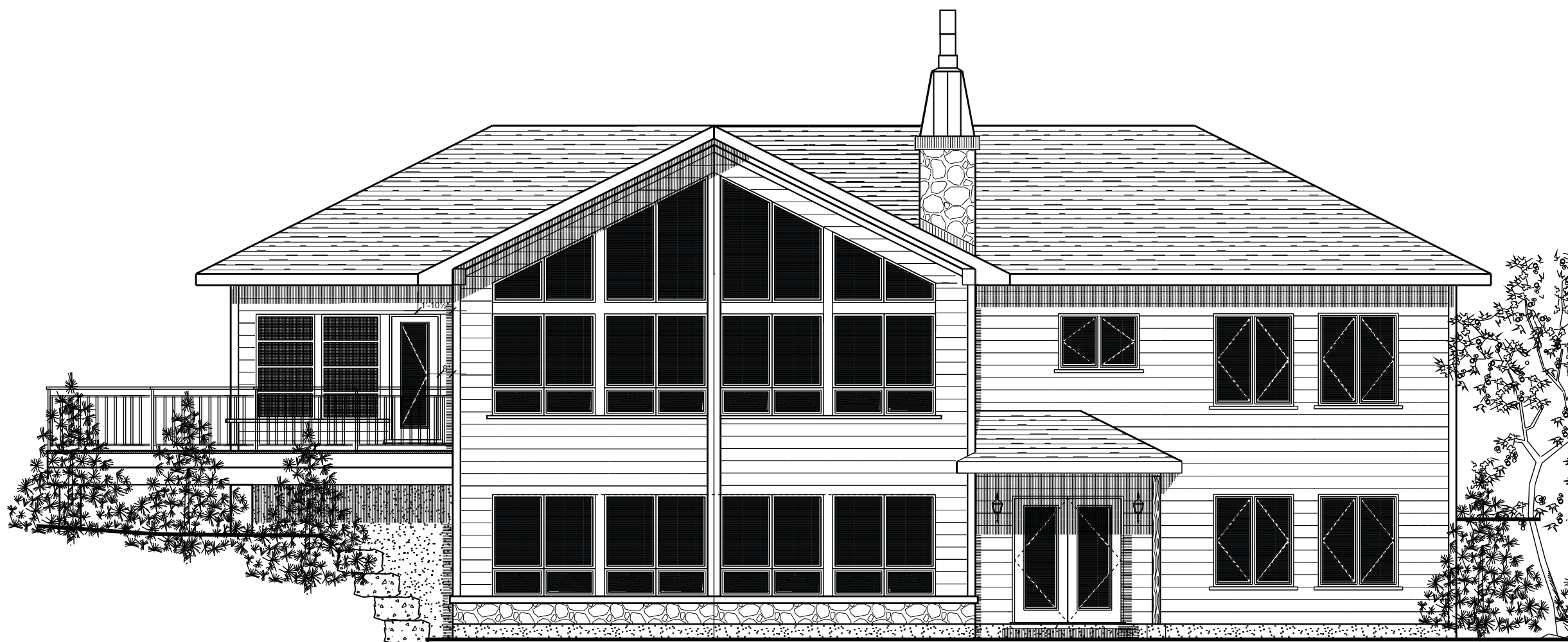
LAKESIDE ELEVATION
